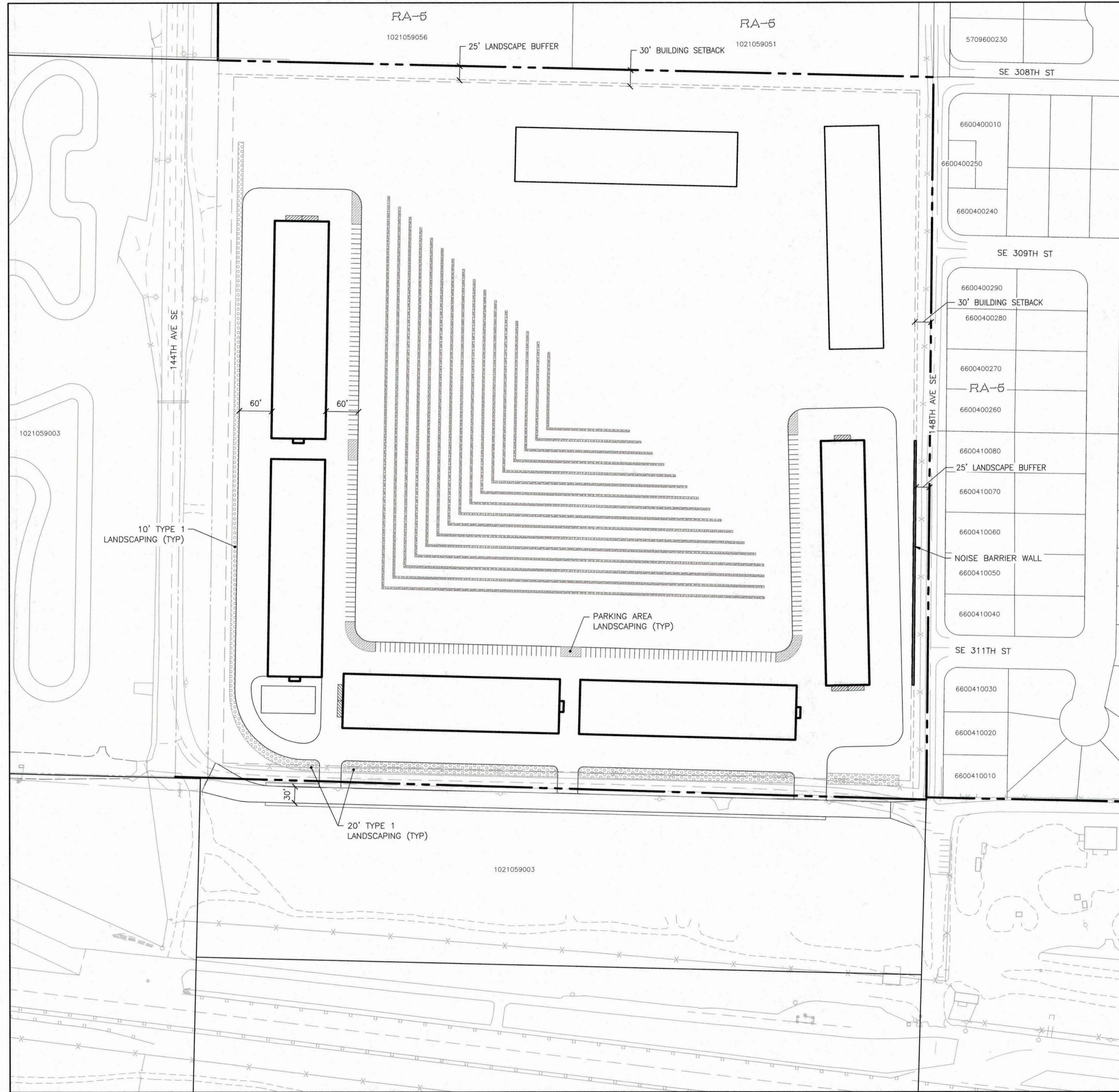
PRELIMINARY LANDSCAPE PLAN SCALE: 1"=100'
