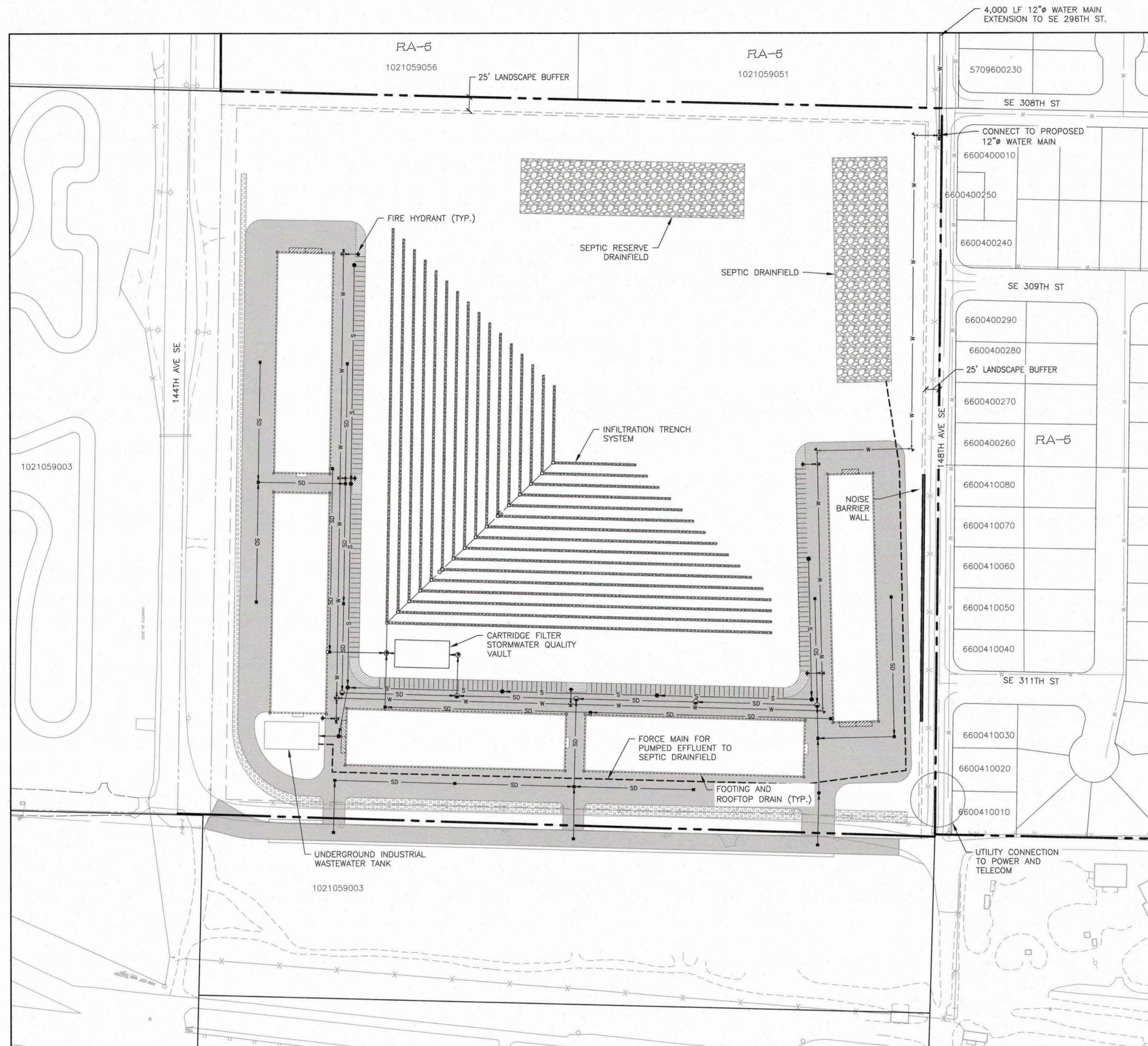
PRELIMINARY UTILITIES PLAN SCALE: 1"=100'
