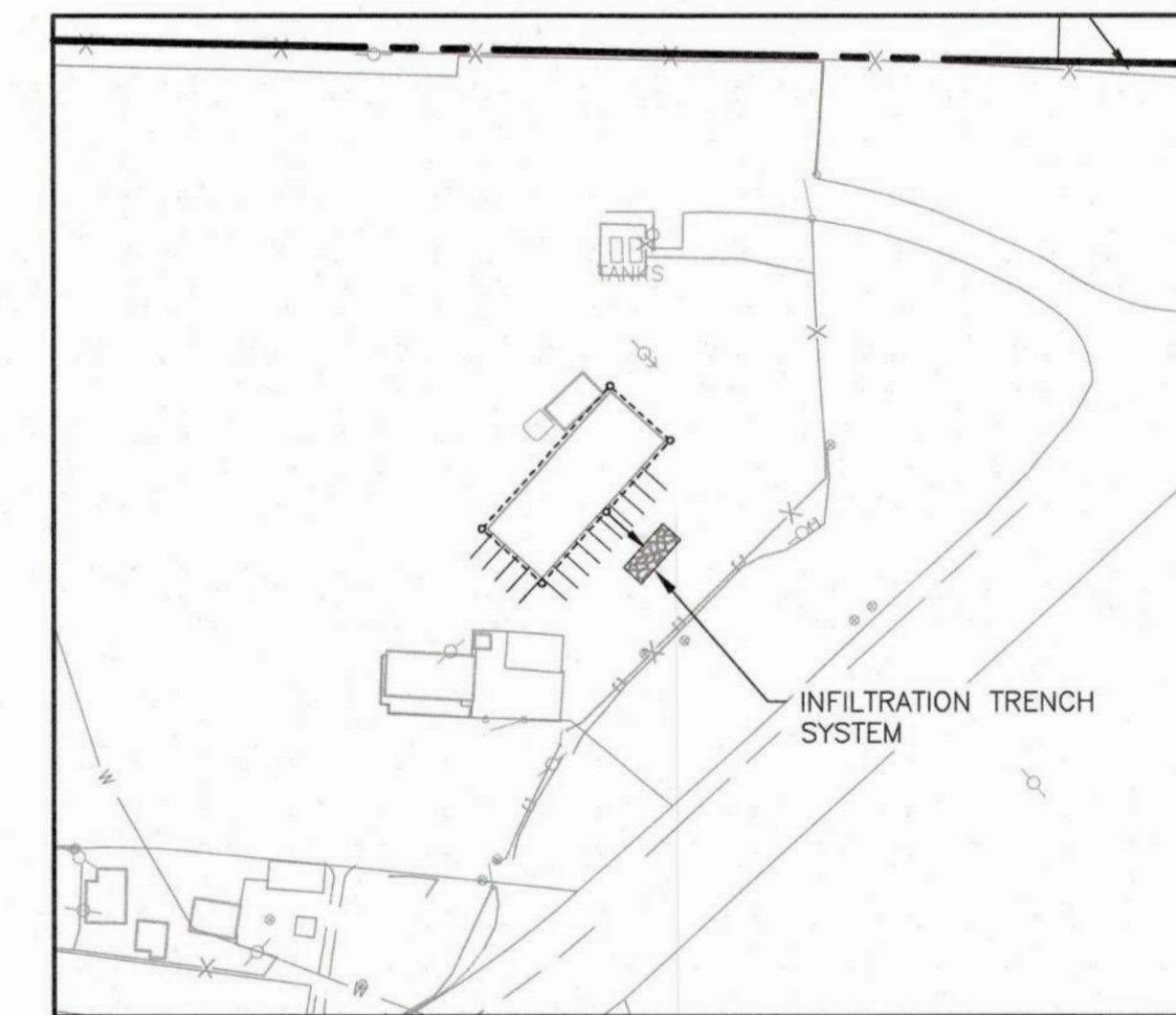
PRELIMINARY UTILITIES PLAN (RETAIL) SCALE: 1"=100'
