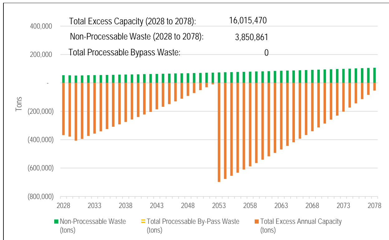
Figure 2–9. Minimize Bypass: Scenario 3, Projected Excess Capacity for 50-Year Planning Horizon
