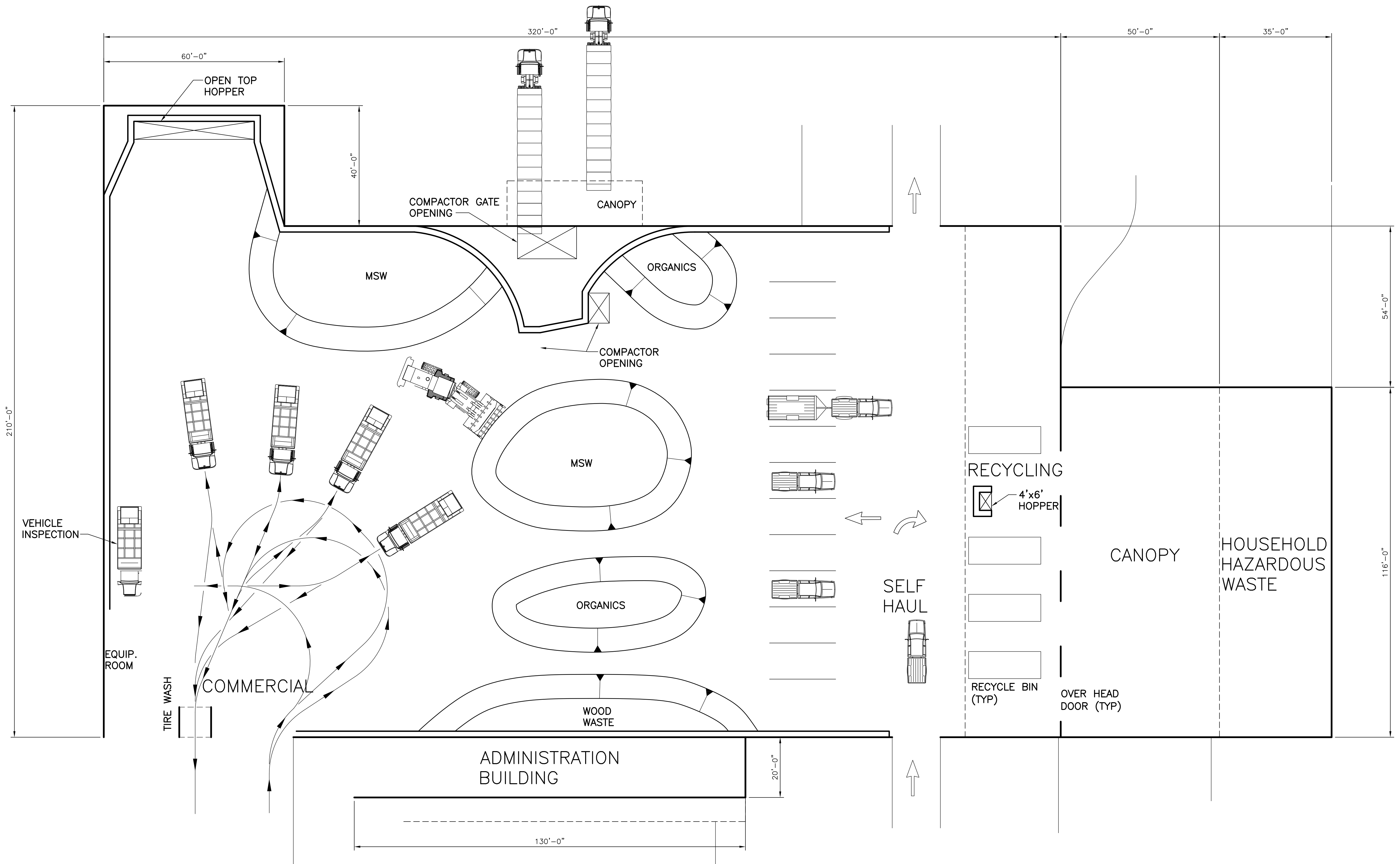
FLOOR PLAN
