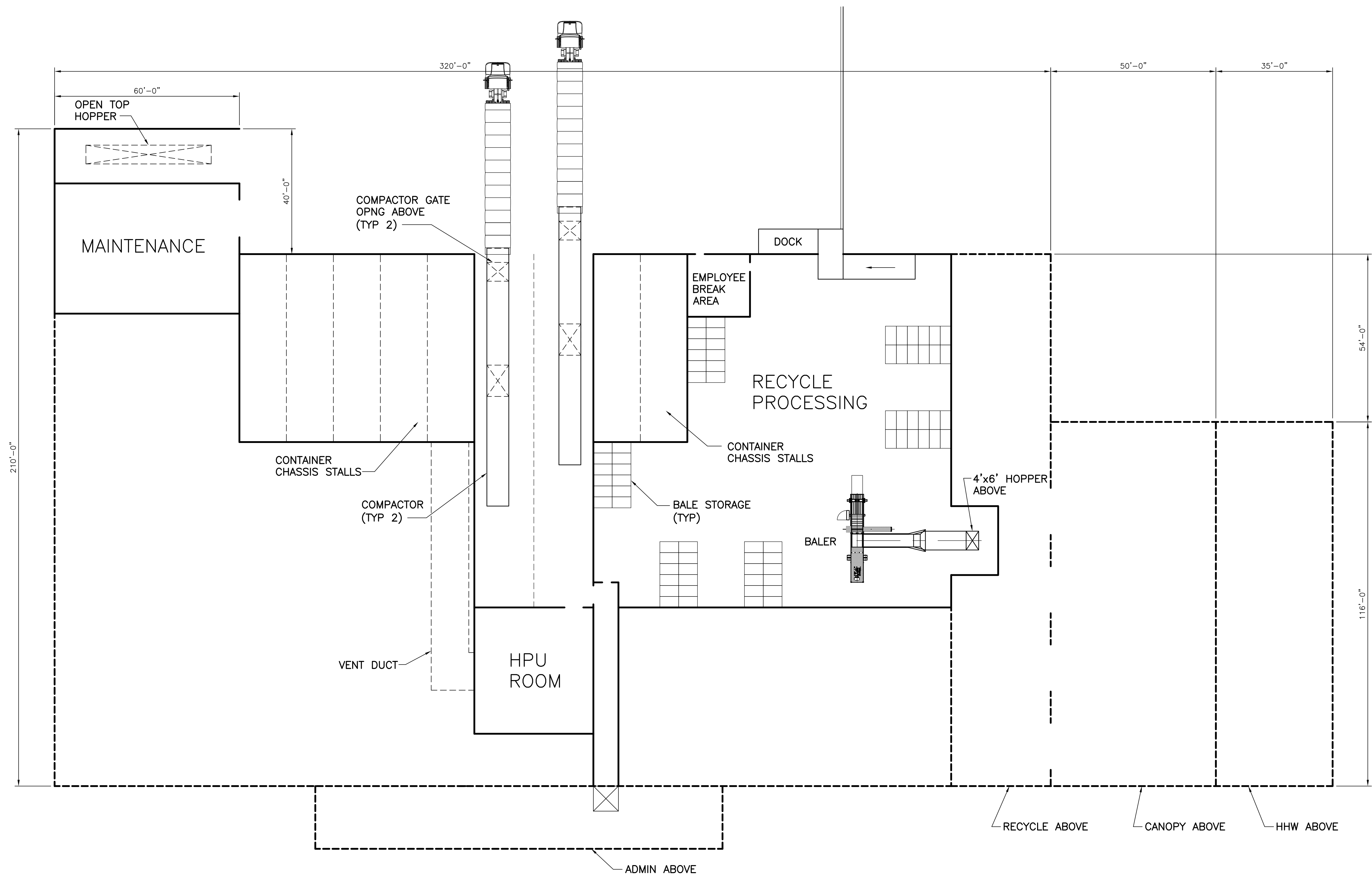
FLOOR PLAN
