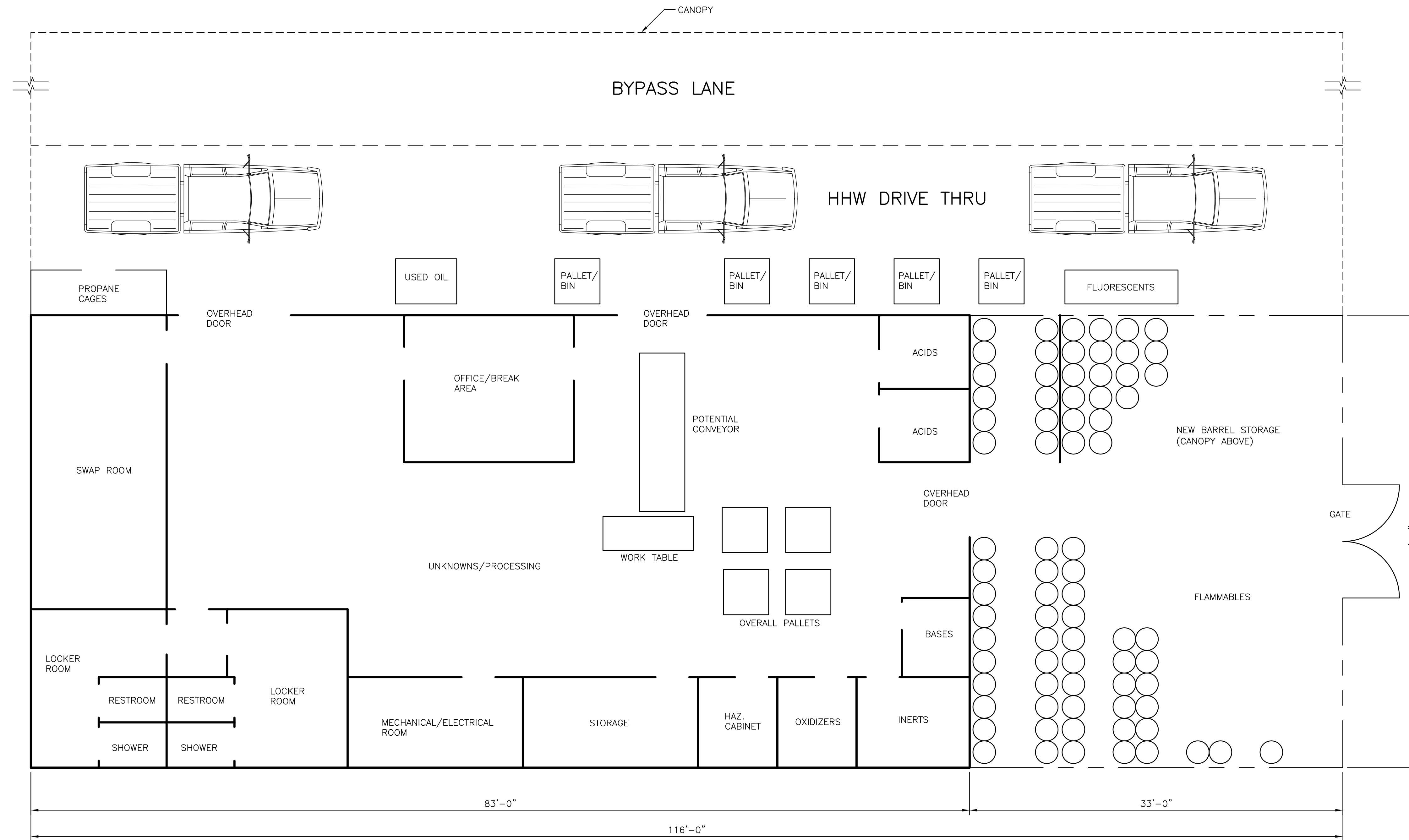
FLOOR PLAN
