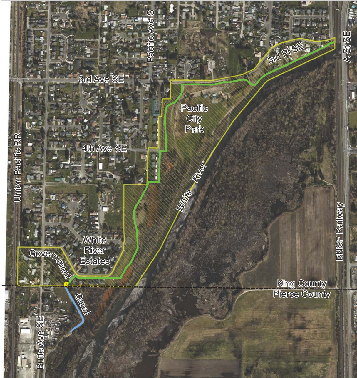
Pacific Right Bank Project - Site Map
