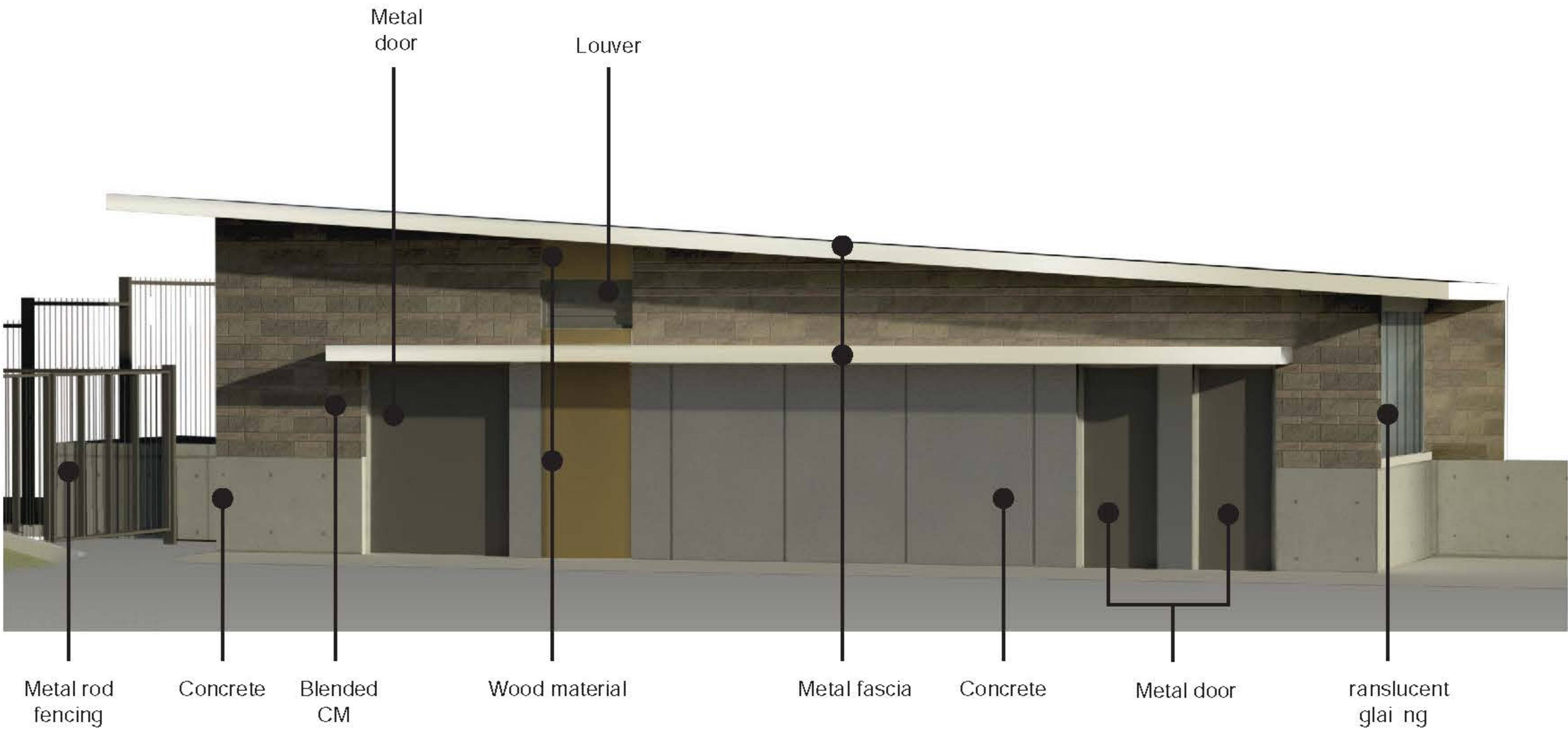
NORTH ELEVATION
