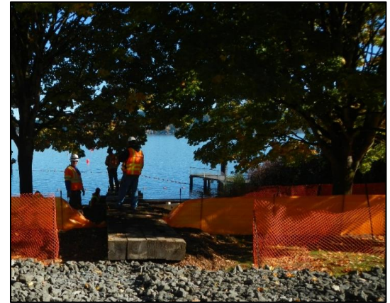
Crews preparing site near the Sunset Pump Station to “float” pipe out on Lake Sammamish.
