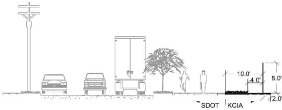
Figure 1: Ellis Ave. Section with Welded Wire fence
